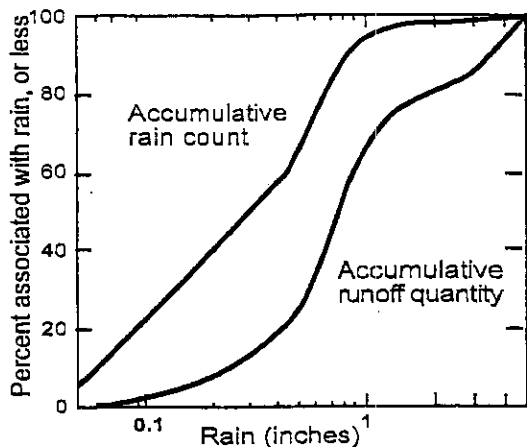
Figure 1.10-4 Milwaukee rain and runoff distributions
