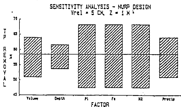
Figure 6.—Sensitivity of model predictions to input factors effects of 2-fold variations in each input factor on predicted phosphorus removal efficiency are shown. Base values are 5 cm for relative volume, 1 m for depth, 650 ppb for P_i , .3 for F_o , and 27 cm for precipitation. For example, the depth bar shows the predicted performance range for a depth range of 0.5 to 2 meters with other input factors held fixed.
