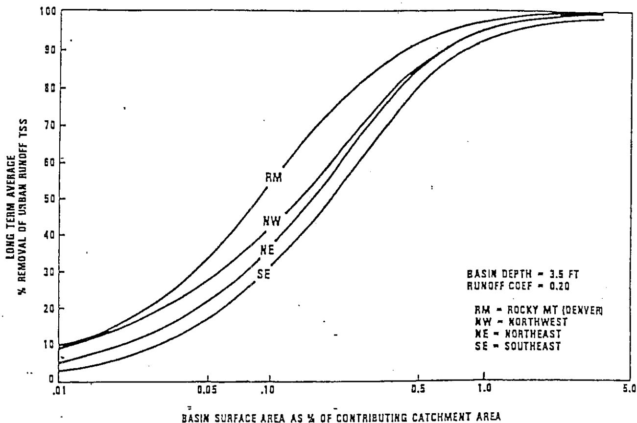
Figure 2.—Detention basin performance for suspended solids removal.
